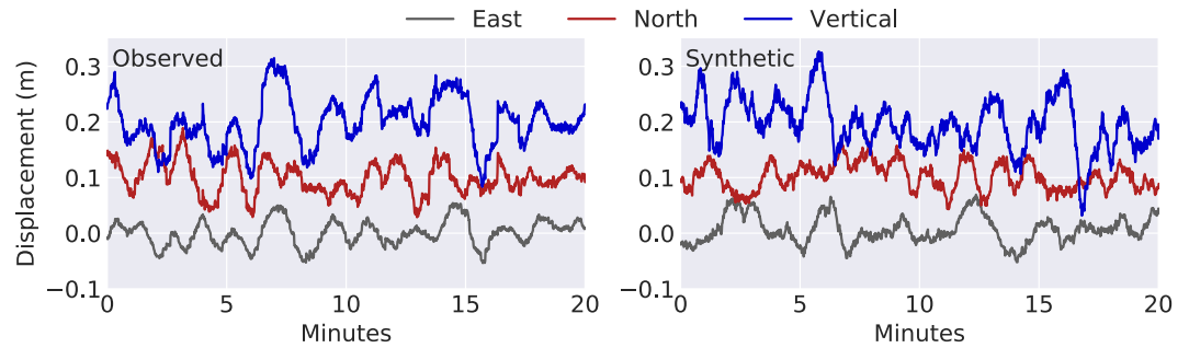
Figure 11. Twenty minutes of noise observed at station BILS (Figure 2) and 20 min of synthetic noise generated using the median noise model from Figure 5. The time series for each direction of motion are offset for clarity.
