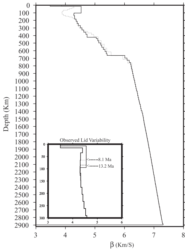
Figure 5. Unique sublid to core-mantle boundary 1-D East Pacific Rise model (EPRM) shear structure used to model all observations of triplicated S^3 , independent of distance from East Pacific Rise ridge axis (solid line). The 255-km-thick transition zone structure adequately accounts for all observed triplication data in Figure 3. Model derived from MELT OBS [Forsyth et al. , 1998] event 345/95 is shown (dotted). Inset shows progressively older sampled plate mandates use of thicker lithospheric lid. Tectonic North America is shown as solid line.
