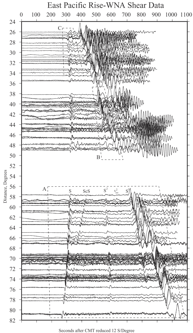
Figure 4. East Pacific Rise shear waveforms in velocity recorded on North American west coast (WNA) broadband networks. Effective aperture of the combined arrays provides upward of 13^\circ of phase move out per event. Data are low-pass-filtered below 5 s. The key structural interpretations are based on modeling of the data shown in boxes; box A contains the S^3 405- and 660-km triplications; box B contains the S^2 660-km triplication; box C contains branch D of the S 660-km triplication.
