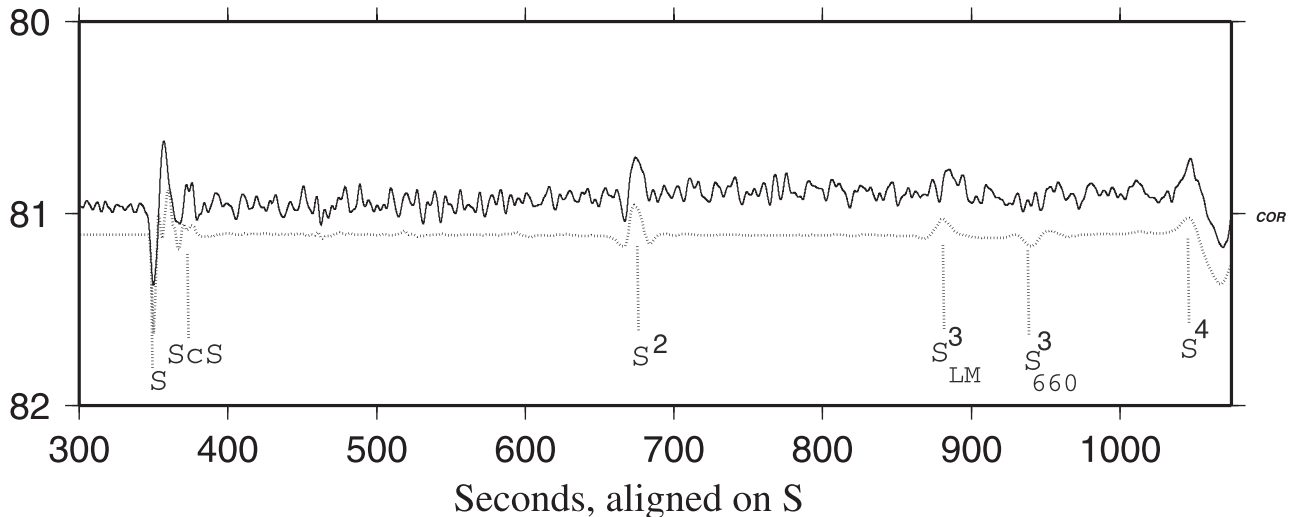
Figure 2. Seismograms in the wide-aperture record section in Figure 4 contain triplicated S , S^2 , and S^3 , in addition to ScS . Despite their teleseismic distances, the triplication phases have propagated entirely in the upper mantle. Simultaneous modeling all of phases across pure path record sections provides a unique one-dimensional model from the CMB to the crust free of depth-velocity ambiguities.
