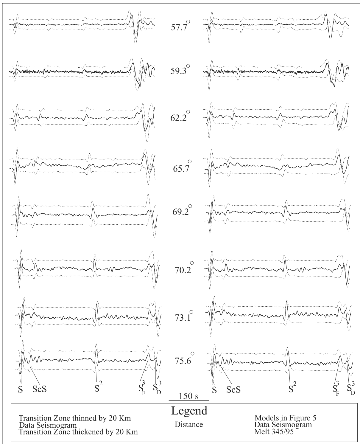
Figure 8. Comparison of other models with the S^3 data. The triplication branches are labeled indicating the crossing of the CD by the F branch of the 660-km triplication. The data are repeated twice at each range; upper right synthetics are our preferred model; lower right is model 345/95 from the recent MELT OBS experiment, derived from subaxial ray paths; top left shows synthetics for a transition zone decreased in thickness by 20 km, bottom left for a 20-km increase in thickness. The crossover of the various phases through the record section cannot be replicated with either of the TZ perturbation models. MELT model 345/95, derived for energy traveling directly under the EPR axis, is significantly slower than the off-axis data discussed here.
