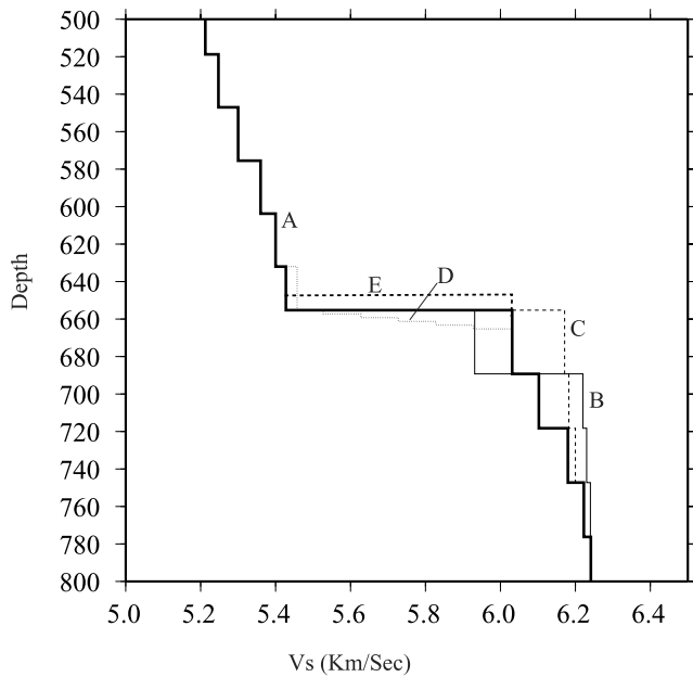
Figure 9. Plots of the 660-km discontinuity structure perturbations with the corresponding waveform fits displayed in Figure 10: model A, the preferred model shown also in Figure 5 for reference; model B, mapping 30% of the 660-km discontinuity into sub-660-km structure, thus removing the high-velocity gradient; model C, increasing the discontinuity jump and removing the underlying gradient; model D, linearly mapping the discontinuity over 25 km radially; and model E, raising the discontinuity to 650 km. Model letters correspond to synthetics profiles of Figures 10a–10e.
