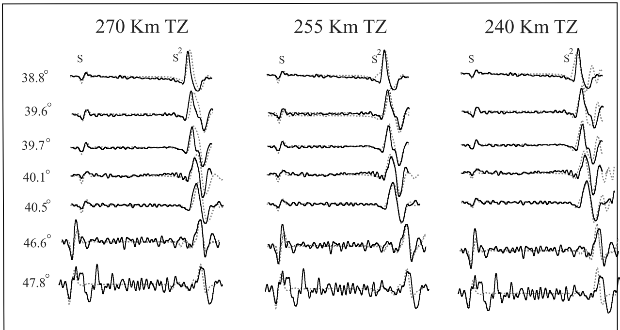
Figure 13. Varying transition zone thickness by 15 km from the best fitting S^3 model, producing misfit in the S^2 arrival time and waveform shape as observed. Increasing TZ thickness by 15 km retards the S^2 arrival at closer distances ( 38^\circ – 40^\circ ), while thinning the TZ by the same amount overly advances the arrival beyond 40^\circ . Best fitting transition zone is not discernibly different than that for the S^3 data traveling 1200 km from the ridge axis.
