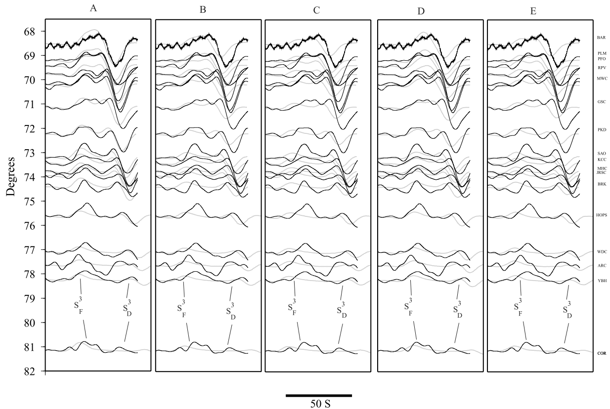
Figure 10. The 660-km triplication phases of S^3 for alternate discontinuity fine structures, aligned on S . These models, shown in Figure 9, produce substantially different waveform fits. (a) Model 1, preferred model, requires the linear gradient to 740 km depth; (b) model B advances the F branch of the 660-km triplication 10+ s beyond that called for by the data; (c) model C overly exaggerates the F-D subphase time separation; (d) model D advances the F branch arrival, again altering the style of F-D phase interference observed in the data between 68° and 72°, as well as overly advancing the back branch of the 660-km reflection beyond 72°. (e) model E, raises the discontinuity by 10 km both, destroying the F-D interference as well as the time separation between the two triplication phases. See text for further analysis of waveform perturbations.
