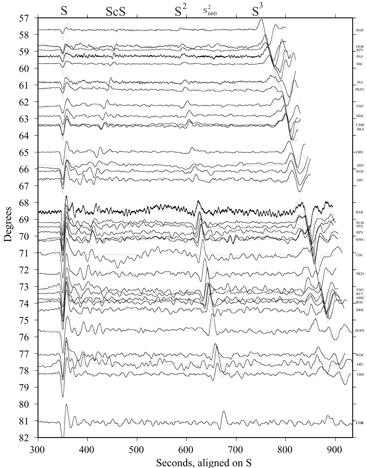
Figure 7. Modeled waveforms containing S , ScS , S^2 , and triplicated S^3 , aligned on S . Regional transition zone thickness variation would be manifested as systematic misfit in subphases of the S^3 triplication, which is not observed. Resolution tests of our ability to assess lid thickness are shown in Figure 8. These data are fit with three different lithospheric lid thicknesses ( V_s 4.55 km/s) shown in Figure 5 (inset). At 57^\circ – 61^\circ (sampling oceanic plate with age 12 Ma), the synthetics are computed with a lid of 73 km, which grows to 76 km for data between 62^\circ and 66^\circ (13Ma). At ranges of 68^\circ – 78^\circ the modeled lid thickness is 58 km thick, reflecting the first surface bounce near the East Pacific Rise ridge crest. The largest misfit in the record section is the ScS phase on stations ARC, WDC, MIN, and ORV, which reflects heterogeneity in D'' (see text). The seismogram from station BAR at 68.5^\circ is unfiltered.
