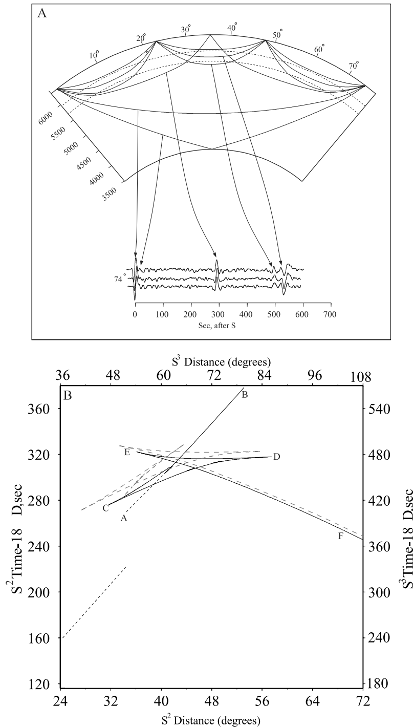
Figure 1. (a) Generalized ray paths showing discrete phases of the upper mantle triplication of multiple (in this case, triple) S . Doubled and tripled time separation of triplicated S^2 and S^3 subphases, respectively, facilitate their slowness identification and synthetic replication relative to S . For the data shown, the AB branch of the 405-km discontinuity triplication is out of range. (b) Triplication plots for the TNA model with (solid) and without (thick dashed) a lid. Fine dashed lines have been added to indicate the position of diffractions. Note that adding a lid does not greatly affect the triplications except to uniformly advance their overall travel times, leaving triplication interference patterns undisturbed.
