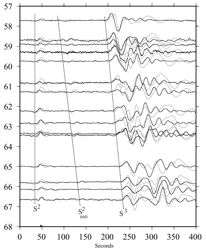
Figure 6. Triplicated S^3 synthetics computed for tectonic North America model, which was derived from paths away from oceanic crust and therefore does not fit oceanic paths. These data are aligned on S , and without a lid both the S^2 phase and the triplicated ensemble of S^3 are late by upward of 10 s due to both their shallower path within the lid and their multiple sampling at surface bounces. With ray parameters similar to S , relative ScS timing at these ranges is insensitive to lid thickness.
